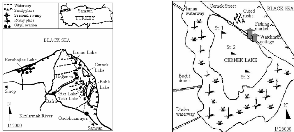
Figure 1. Geological situation of Kızılırmak Delta and sampling stations.
