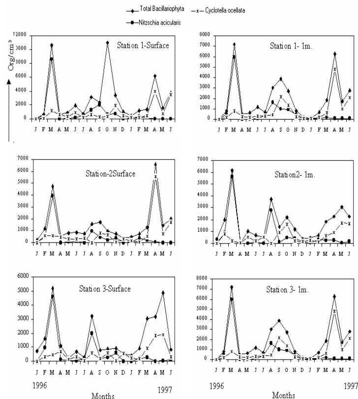
Figure 3. The seasonal variations of total Bacillariophyta, Cyclotella ocellata and Nitzschia acicularis in all sampling stations.
