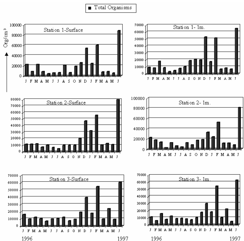
Figure 2. The seasonal variations of total organisms/cm 3 in the sampling stations.
